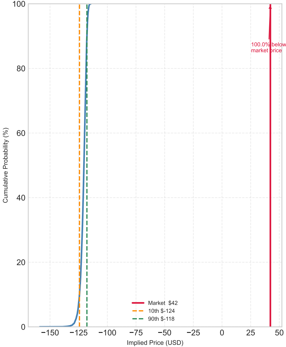
Cumulative Distribution
